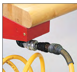
Air or fluid power Each bench has 4 knockouts for Air or Fluid power. Knockouts are in both top and bottom of leg.
