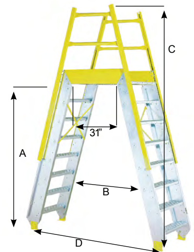
Ship's Ladder Crossover Bridge
